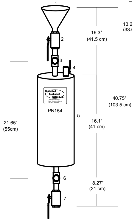
Base Model
