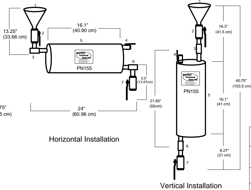
Offset Model
